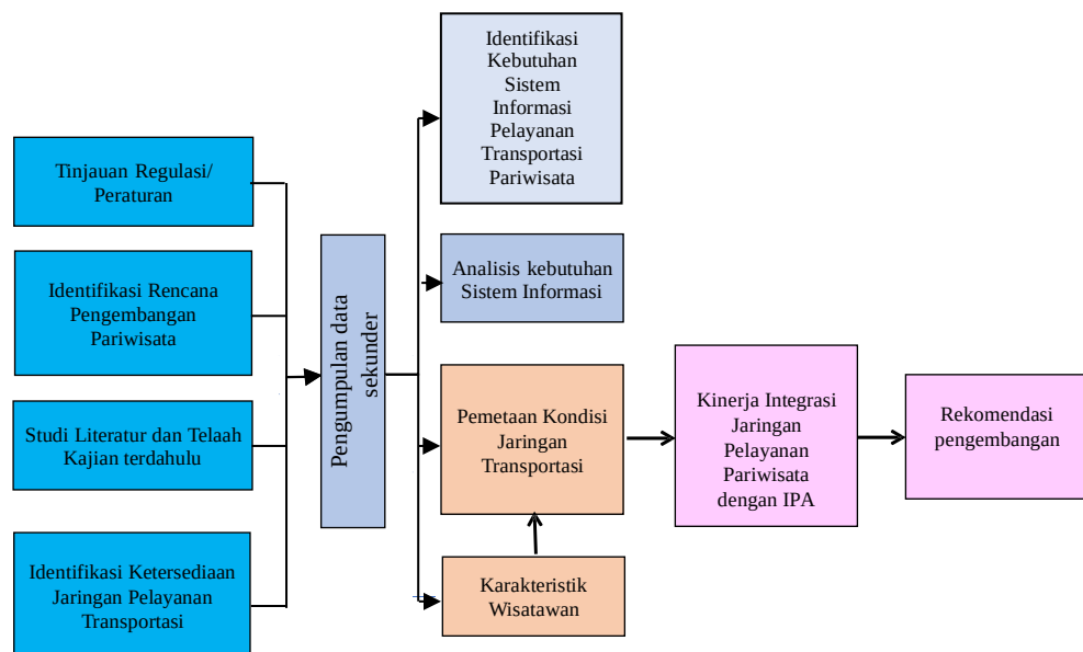
Gambar 1. Framework penelitian
