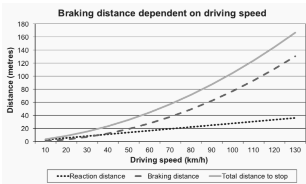
Figure 10 Braking distance dependent on driving speed
