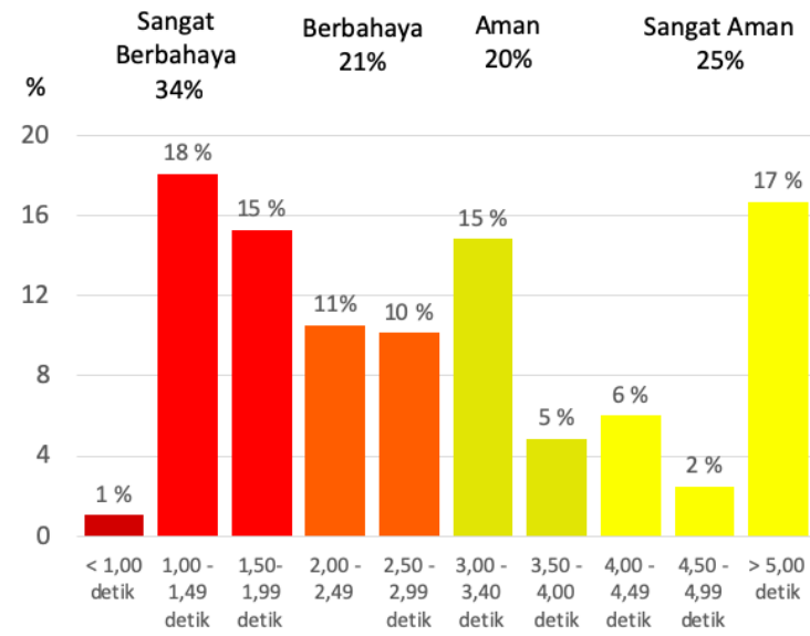
Figure 9. Vehicle Headway Distribution
