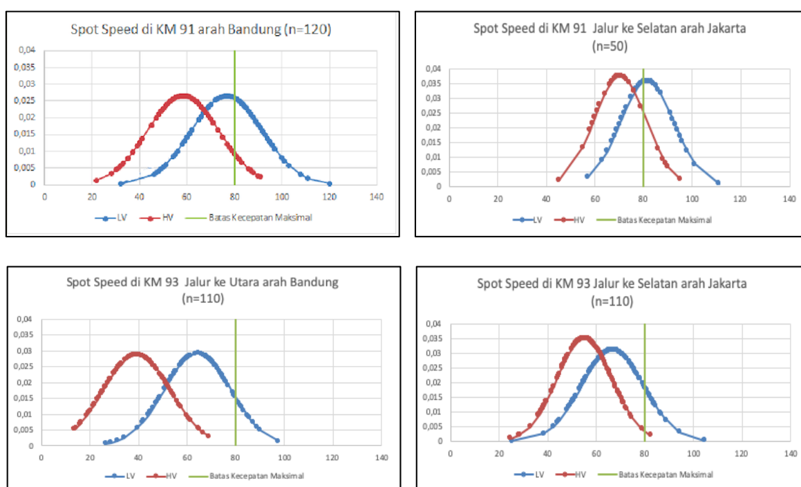
Figure 7. Observed speed distribution
