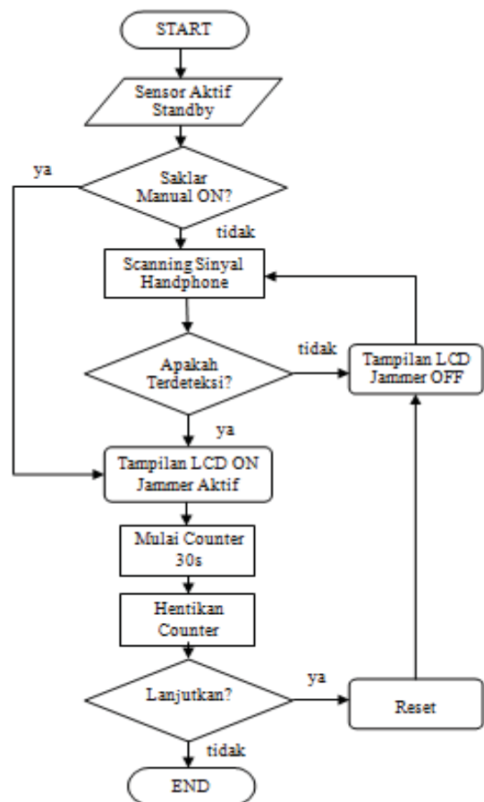
Gambar 3. Flowchart Sistem
