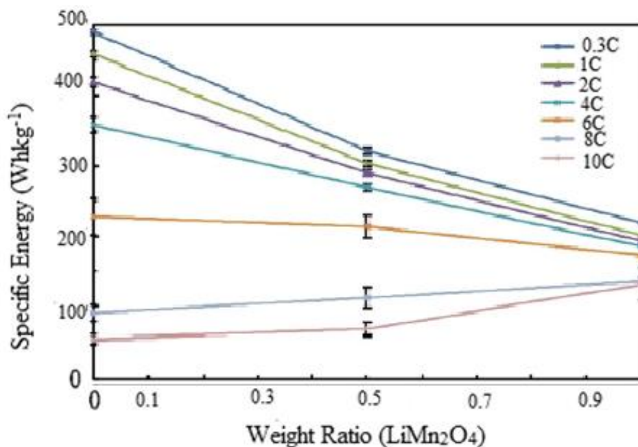
Figure 8. Specific energy versus weight ratio at different discharge rates
