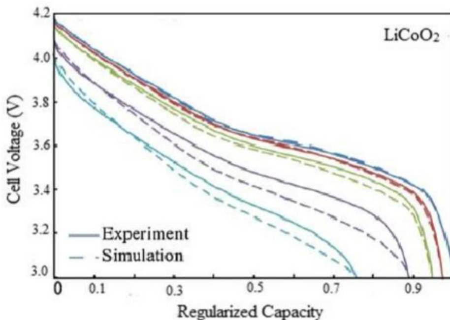
Figure 5. Cathode formulated \text{LiCoO}_2 blended experimental and simulation rate performance
