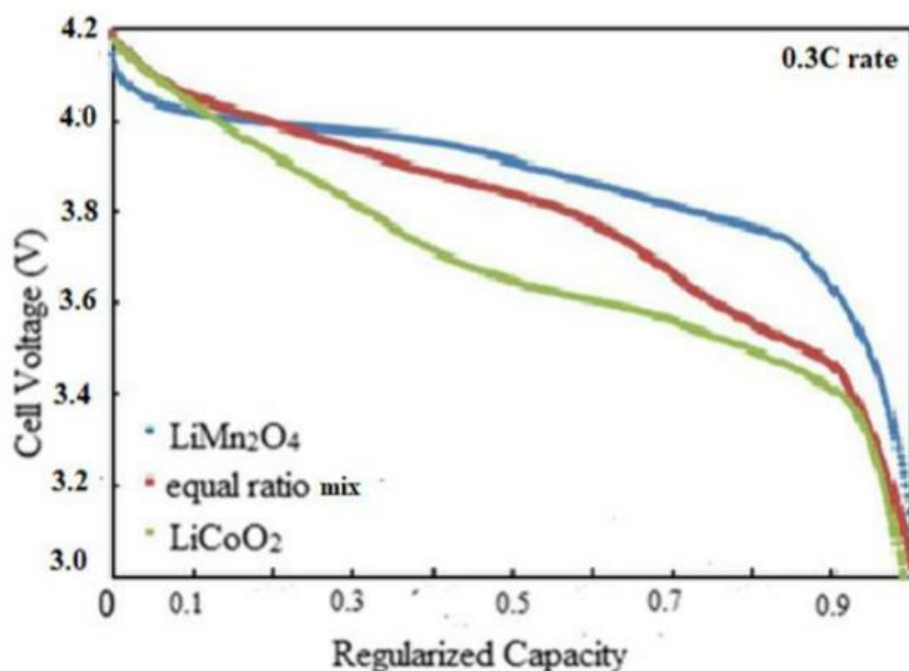
Figure 4. Cathode electrode discharge profiles from experimental results consisting unblended \text{LiMn}_2\text{O}_4 , \text{LiCoO}_2 and equal ratio of the mix at 0.3C rate
