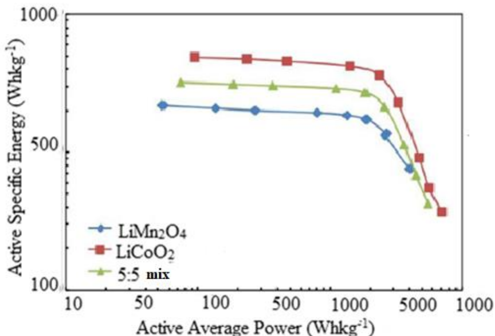
Figure 9. Ragone plot for the various cell compositions
