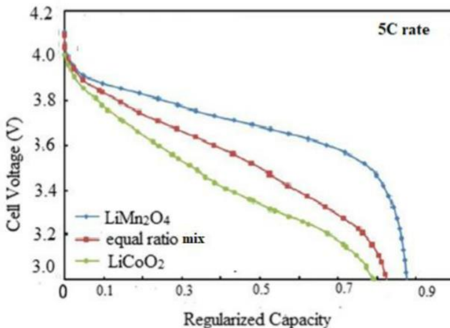
Figure 3. Cathode electrode discharge profiles from experimental results consisting unblended \text{LiMn}_2\text{O}_4 , \text{LiCoO}_2 and equal ratio of the mix at 5C rate
