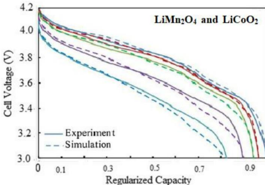
Figure 7. Cathode formulated \text{LiMn}_2\text{O}_4 and \text{LiCoO}_2 blended experimental and simulation rate performance for 5:5 weight ratio at 0.3C, 0.6C, 1C, 2C and 4C
