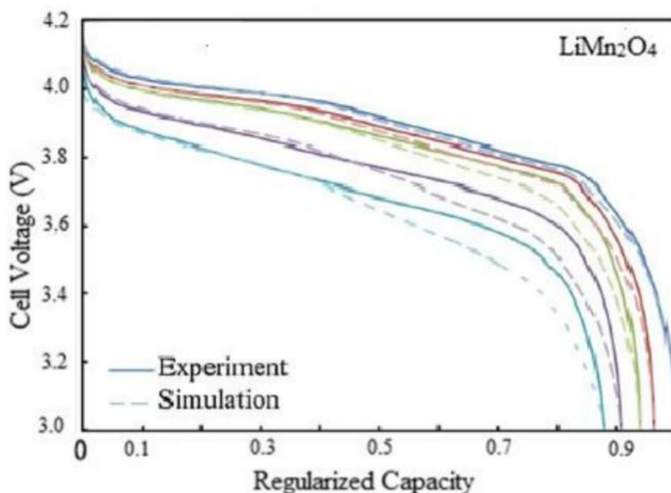
Figure 6. Cathode formulated \text{LiMn}_2\text{O}_4 blended experimental and simulation rate performance
